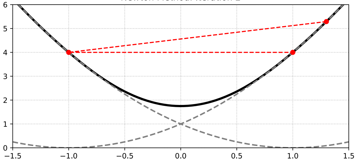
Newton Method: Iteration 2
