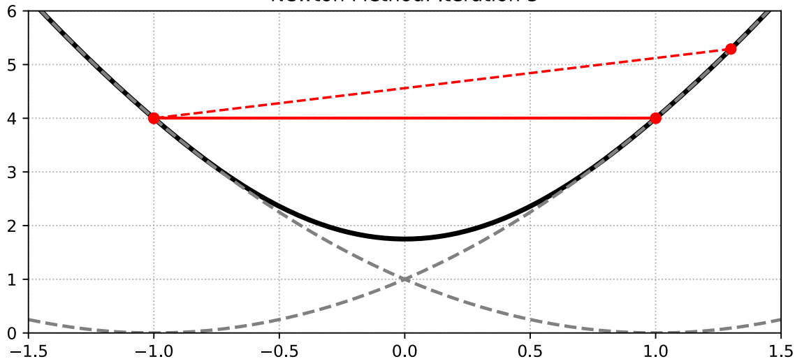
Newton Method: Iteration 5
