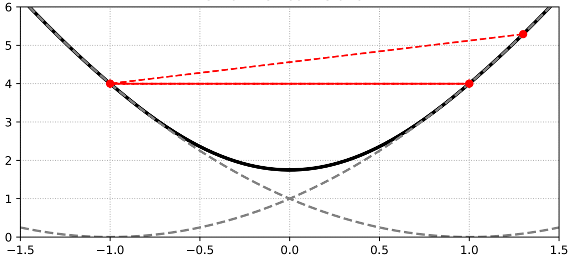
Newton Method: Iteration 4
