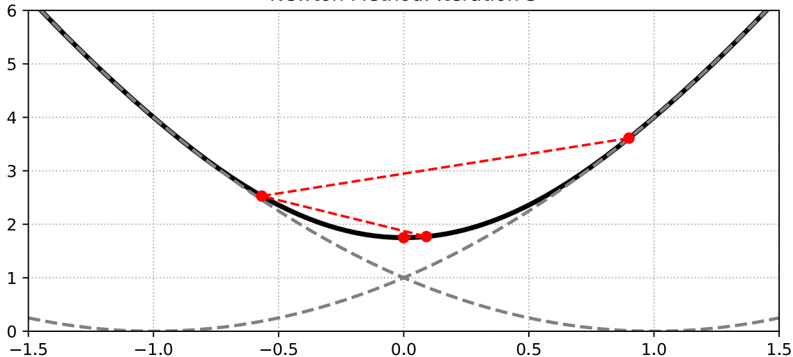
Newton Method: Iteration 3
